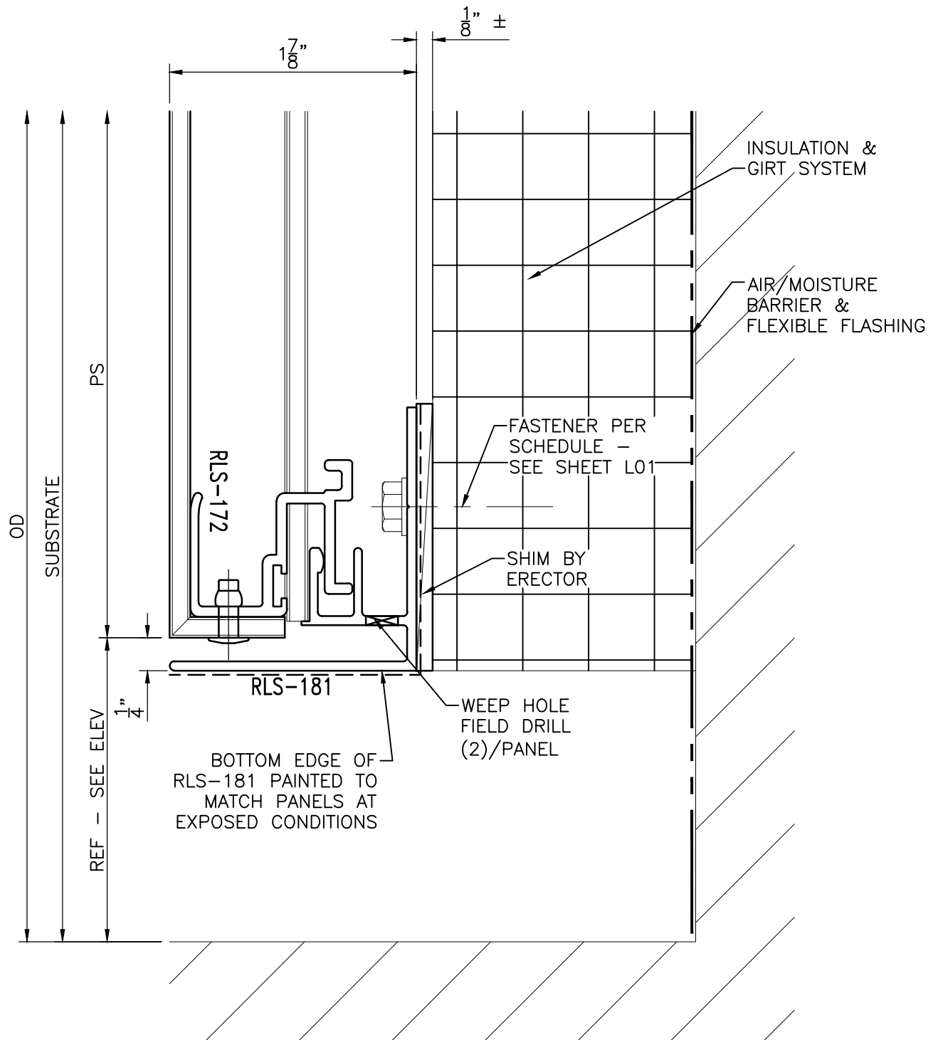
TYPICAL SILL (EXPOSED)
